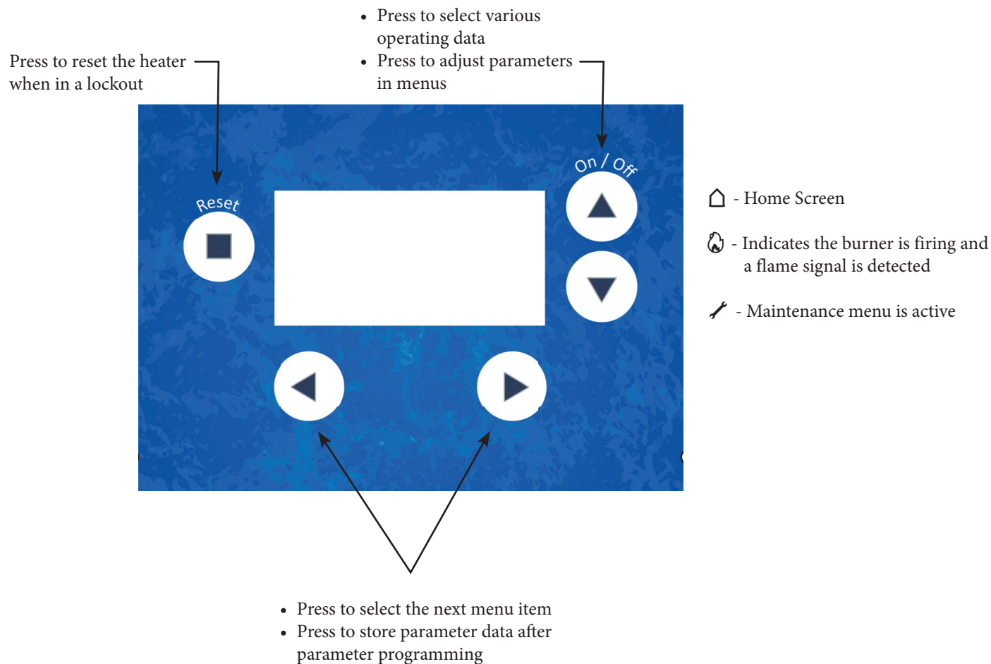
Figure 3-1_ Control Panel
